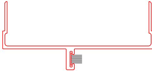
CW 93-10-1 ADF HEADER DEMOUNTABLE
